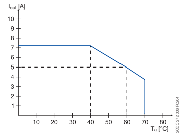
Temperature curve at U_{out} = 24 V DC
