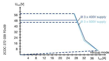
CP-T 48/20.0 (preliminary curve)
