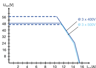
CP-T 48/10.0 U/I curve
