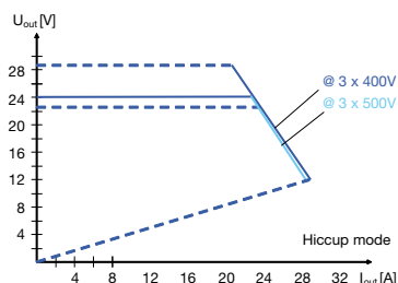
CP-T 24/20.0 Hiccup mode
