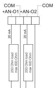
M2M I/O analogue outputs
