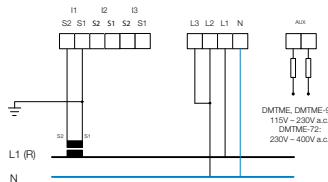
Single-phase system with neutral and 1 CT
