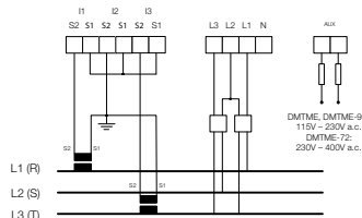
Three-phase system with 2 CTs and 2 VTs (Aron)
