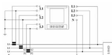
Insertion with 3 CTs
