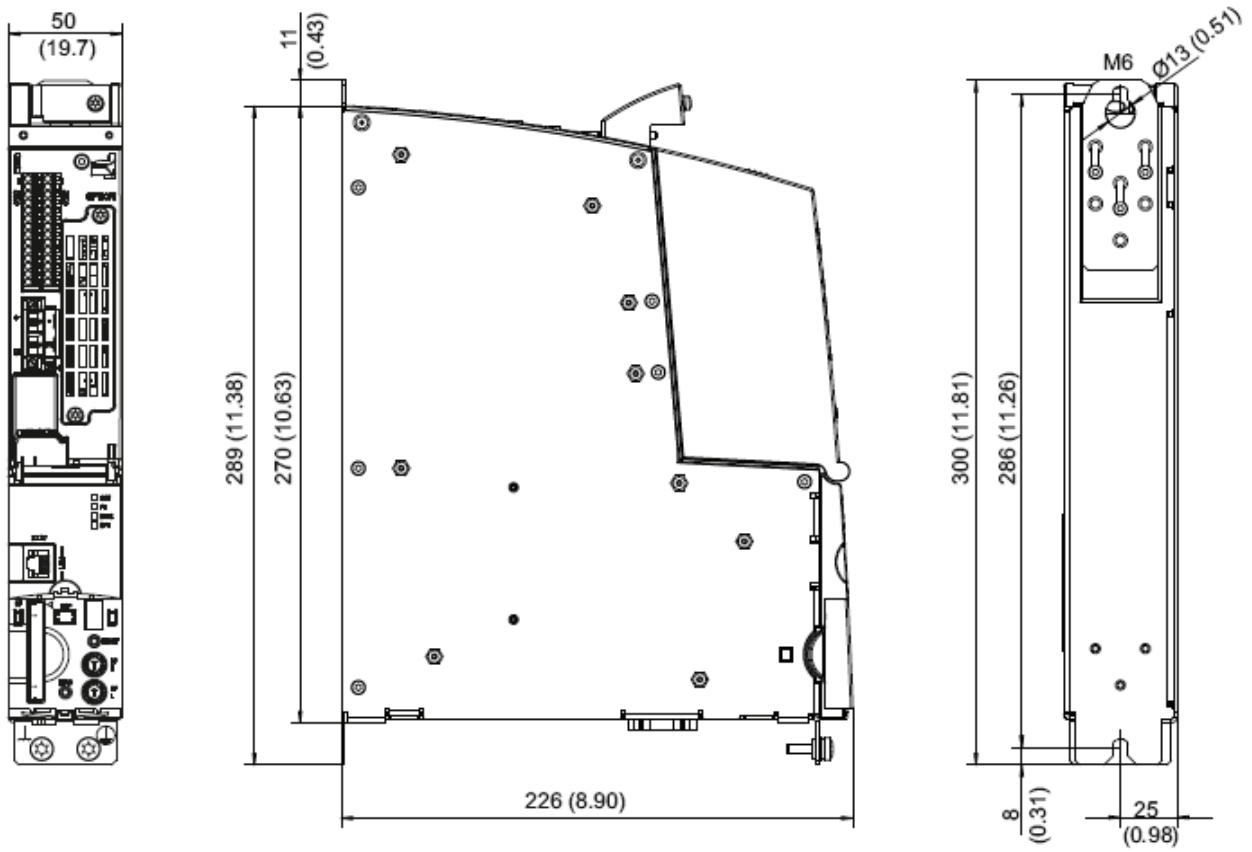
Dimension drawing of the Control Unit CU320-2 PN (Order No 6SL3040-1MA01-0AA0)
