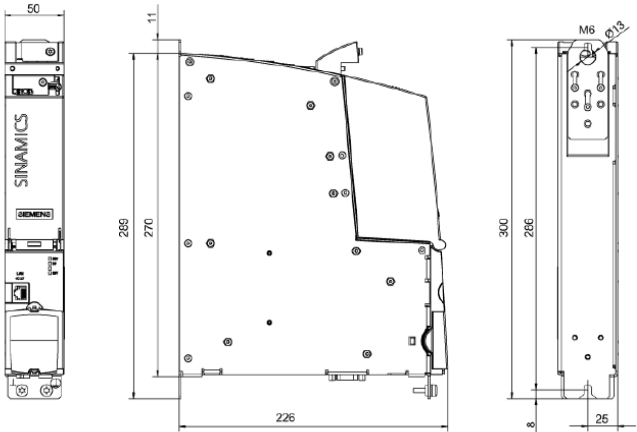
Dimension drawing of the Control Unit CU320-2 DP (Order No 6SL3040-1MA00-0AA0)
