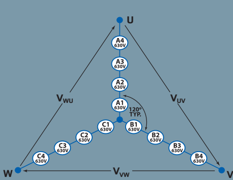
Equivalent Circuit of 4-Cell Generation 3 ROBICON Perfect Harmony Drive with all cells in service • 4160 Volts Type. (Line-to-Line)
