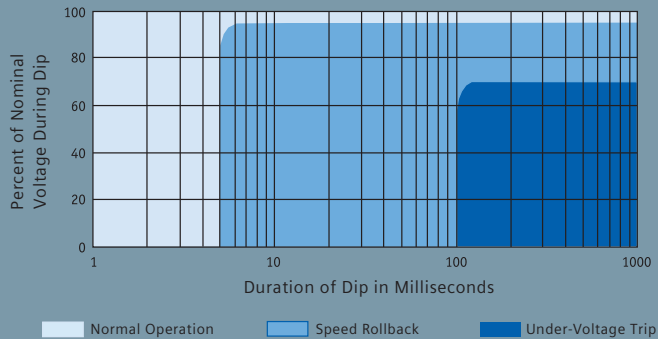
Voltage Dip Withstand Capability During Full Load, Nominal Voltage
