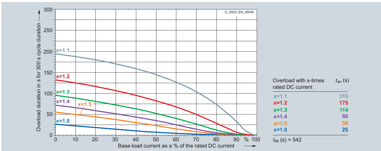
6RA8087-6DS22-0AA0 850 A/two-quadrant operation 400 V, 6RA8087-6FS22-0AA0 850 A/two-quadrant operation 480 V
