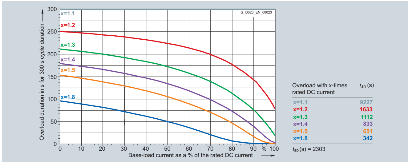
6RA8013-6DV62-0AA0 15 A/four-quadrant operation 400 V, 6RA8013-6FV62-0AA0 15 A/four-quadrant operation 480 V
