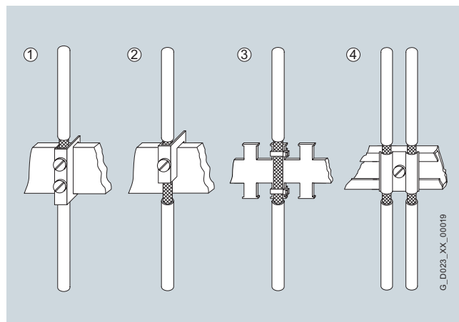
Shield connection
