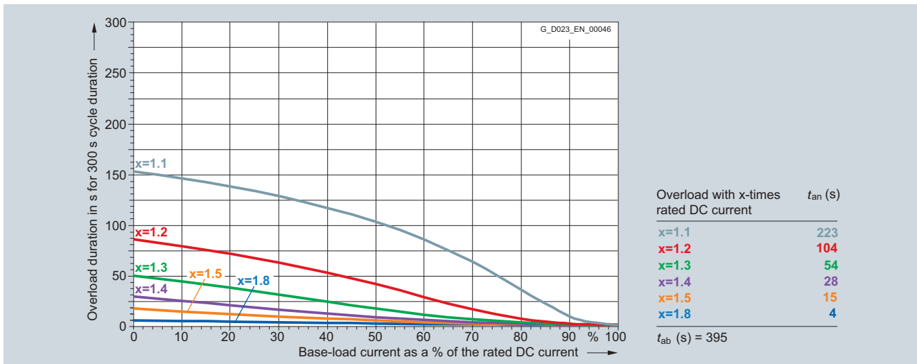
6RA8091-6DS22-0AA0 1 200 A/two-quadrant operation 400 V, 6RA8091-6FS22-0AA0 1 200 A/two-quadrant operation 480 V, 6RA8091-6FV62-0AA0 1 200 A/four-quadrant operation 480 V, 6RA8091-6DV62-0AA0 1 200 A/four-quadrant operation 400 V
