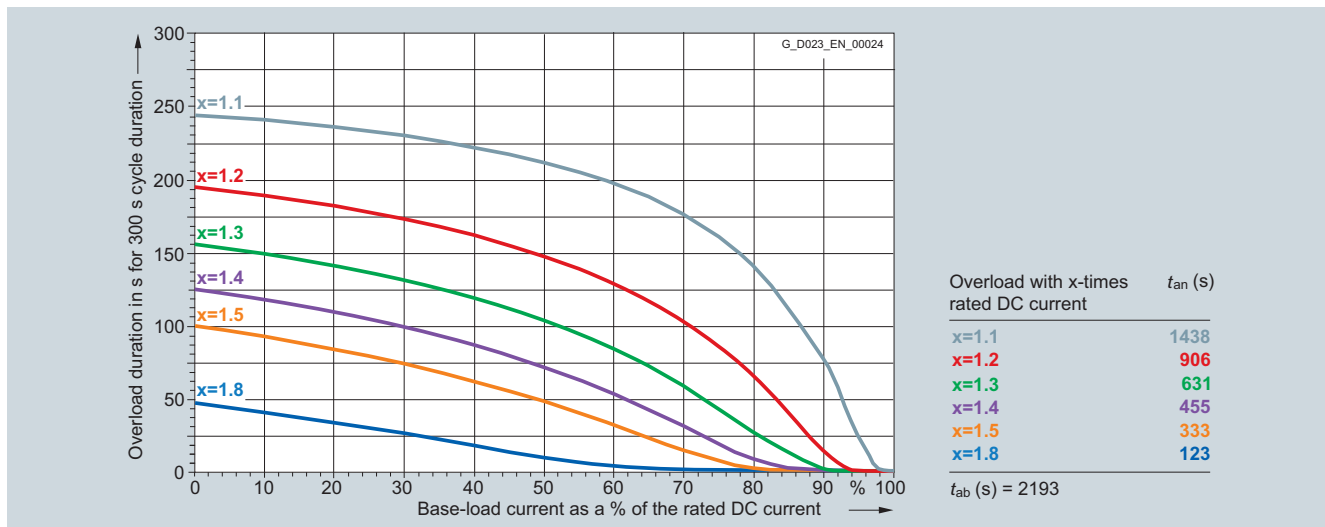
6RA8018-6DV62-0AA0 30 A/four-quadrant operation 400 V, 6RA8018-6FV62-0AA0 30 A/four-quadrant operation 480 V
