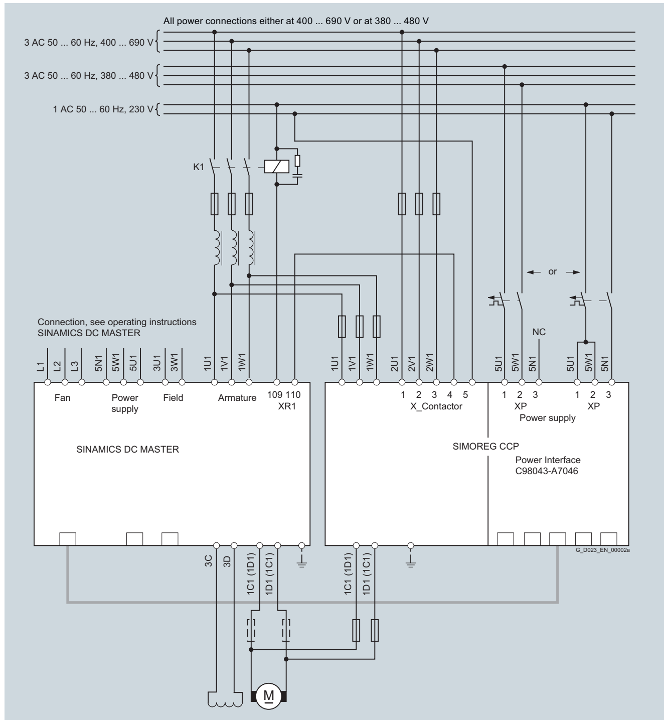
Block diagram
