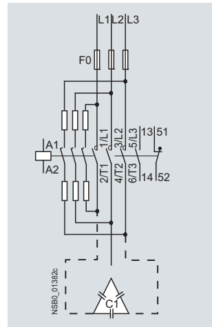
Size S00
