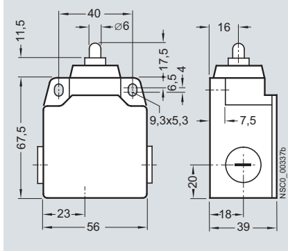
Rounded plunger, type B
