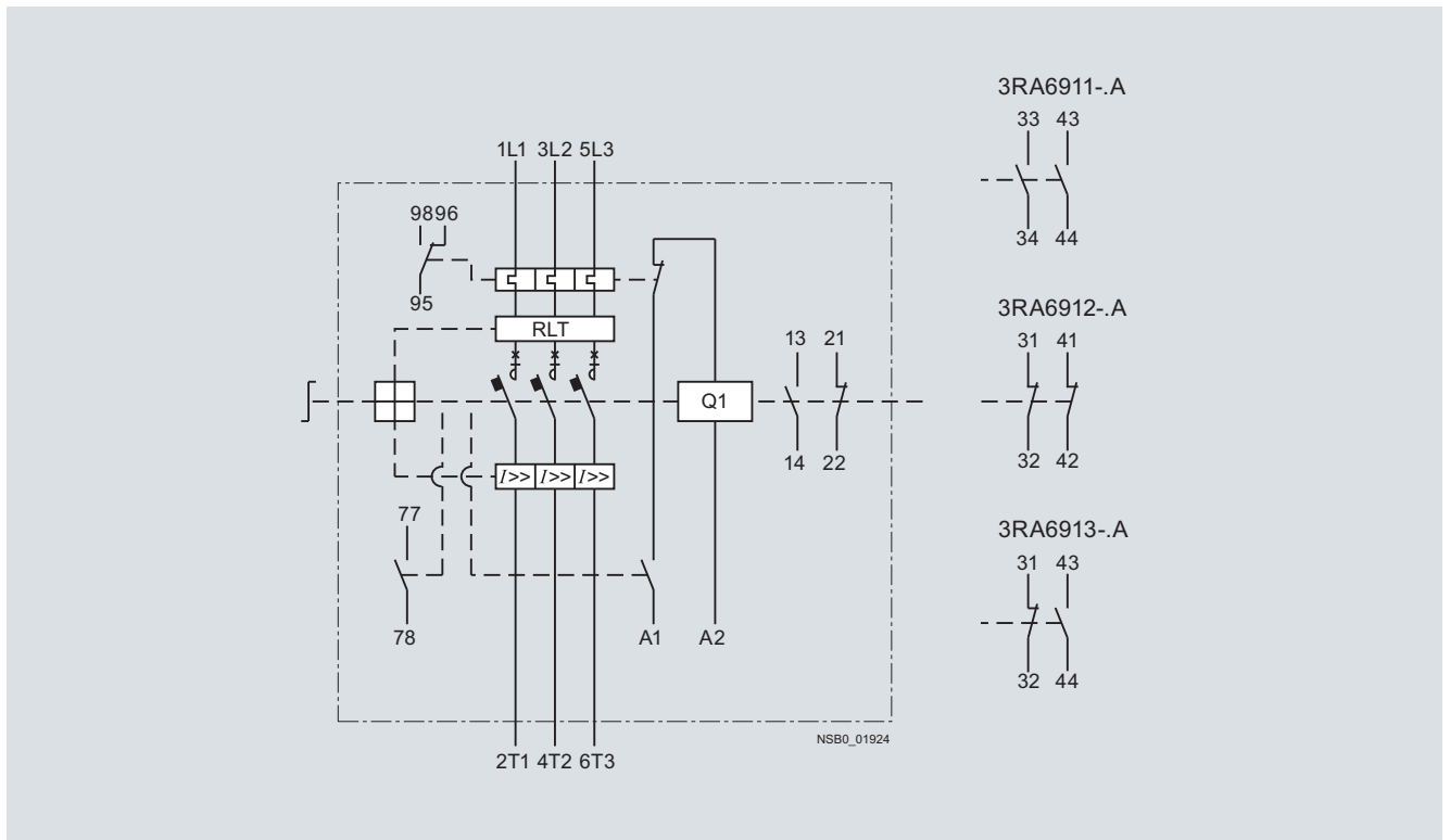
Schematic for 3RA61 direct-on-line starters (main circuit)
