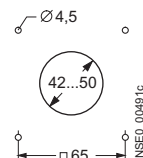
Door cut-out with mounting holes
