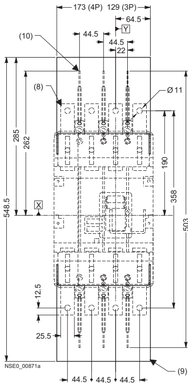
Hole pattern for plug-in base with front connecting bars
