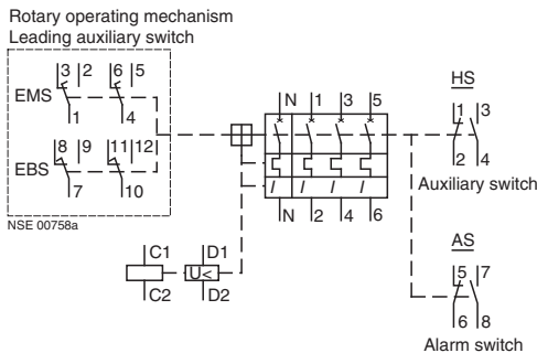
Connection diagram for SENTRON VL160X (3VL1) to VL630 (3VL5), 3- and 4-pole circuit breakers for system protection with thermal-magnetic overcurrent releases
