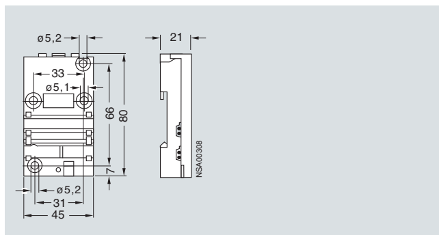
AS-Interface standard distributor, for AS-Interface flat cable (3RK1 901-1NN00)
