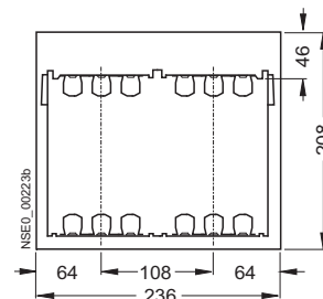
3NY7 502 molded-plastic masking frame for two 3NP40 switch disconnectors for installation in ALPHA distribution boards
