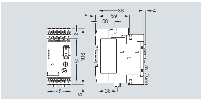
3RB29 06-2BG1, 3RB29 06-2DG1 current measuring module
