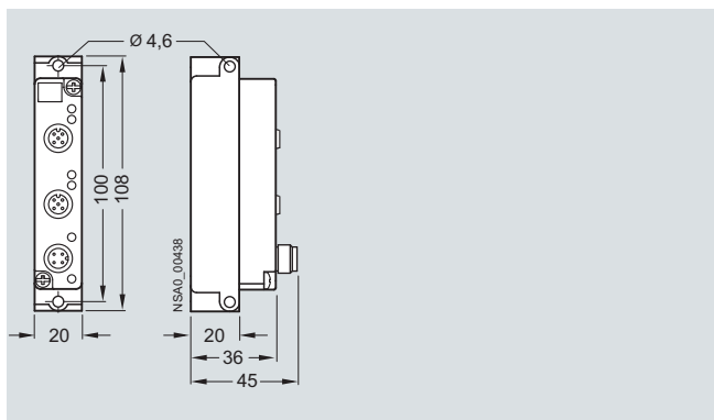
K20 module, four inputs, M12 (3RK2 200-OCQ30-0AA3) K20 module, two inputs/two outputs, M12 (3RK2 400-1BQ30-0AA3) K20 module, two safety inputs, M12 (3RK1 205-0BQ30-0AA3)
