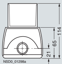
Enclosure with protective collar, metal
