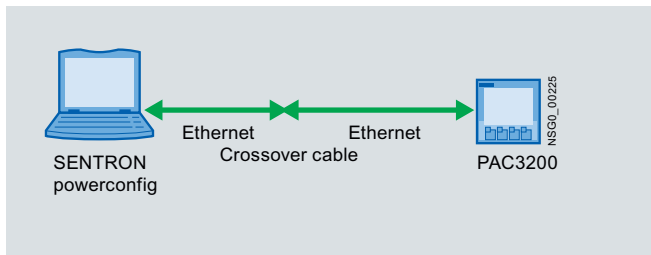
Direct connection between the PC and PAC3200
