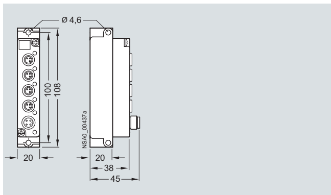
K20 module, four inputs, M8 (3RK2 200-OCT30-0AA3) K20 module, two inputs/two outputs, M8 (3RK2 400-1BT30-0AA3)
