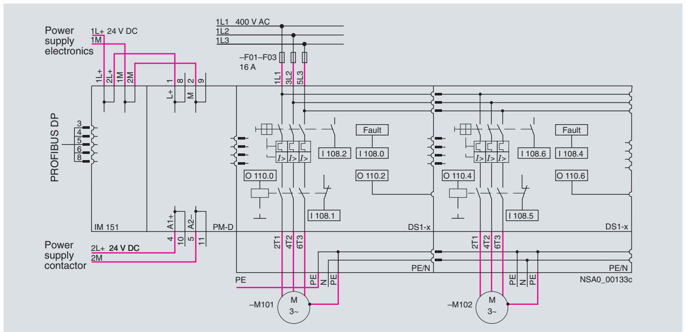
Sample illustration of an ET 200S station with PM-D power module and two standard motor starters
