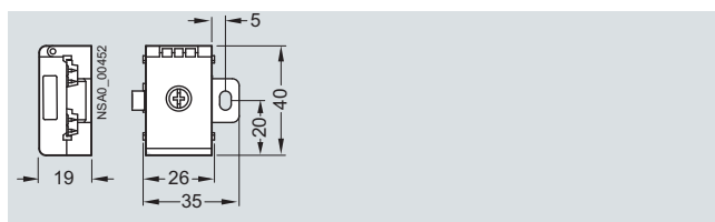
AS-Interface compact distributor, for AS-Interface flat cable (3RK1 901-1NN10)
