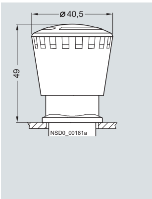
EMERGENCY-STOP mushroom pushbutton with rotate-to-unlatch mechanism
