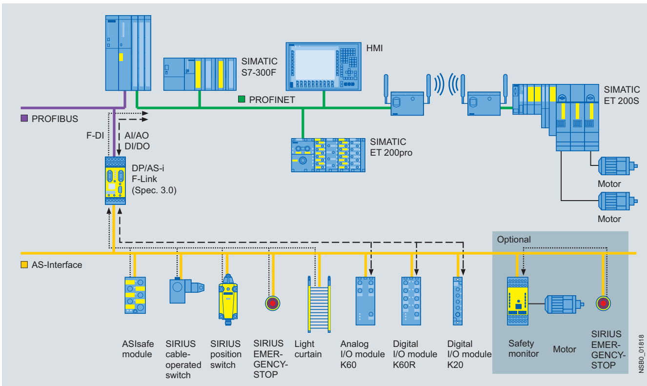
Integration in PROFINET networks under SIMATIC F PLC (alternatively can also be integrated through IE/PB Link)
