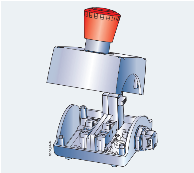
EMERGENCY-STOP enclosure
