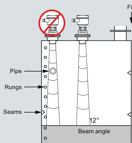
Pointek ULS 200 Mounting
