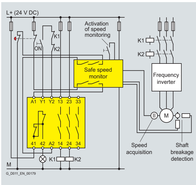
Conventional wiring
