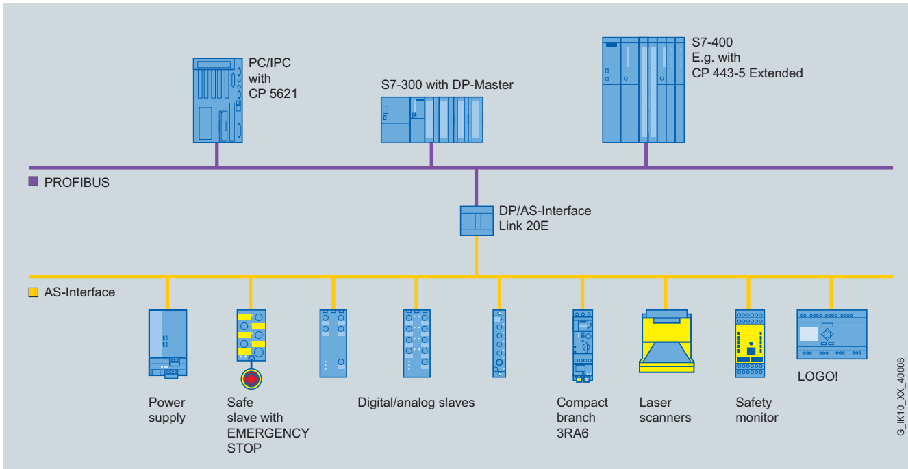
Transition from PROFIBUS DP to AS-Interface using DP/AS-Interface Link 20E
