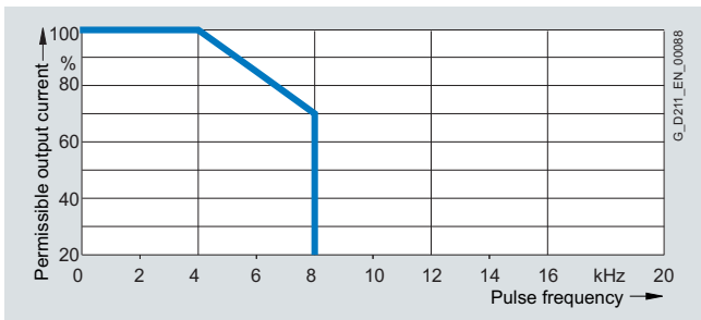
Output current as a function of pulse frequency
