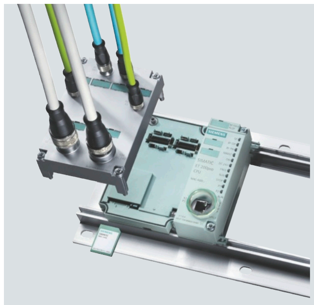
Interface module and connection module
