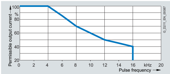
Output current as a function of pulse frequency
