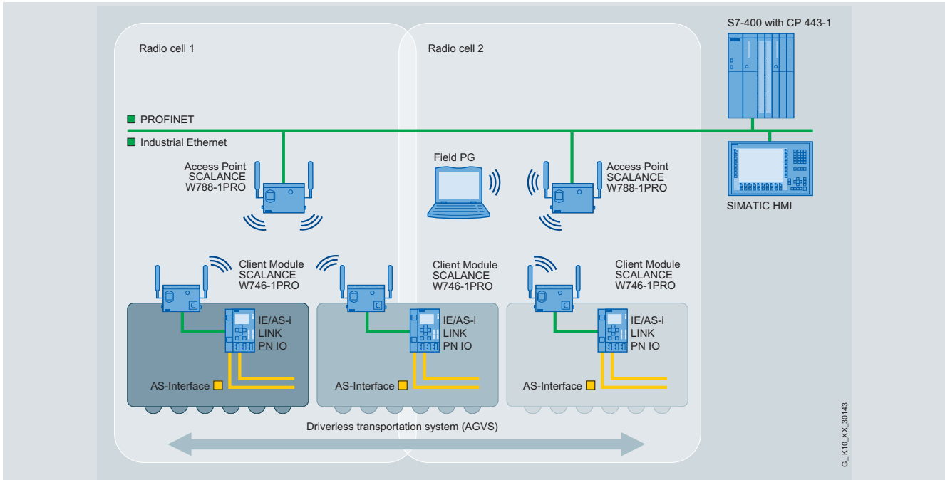
Wireless communication between Industrial Ethernet and AS-Interface components
