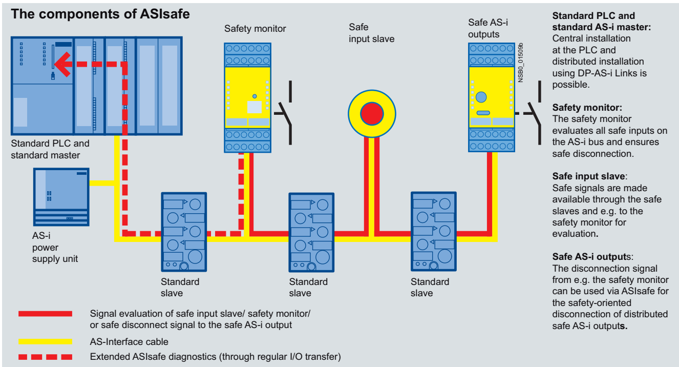
The ASIsafe components and their signal flows
