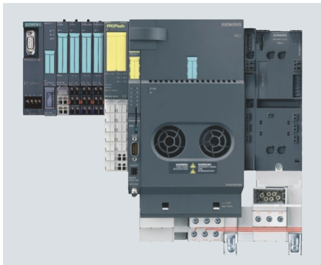
Design of an ET 200S station with two ET 200S FC fail-safe frequency converters (on the right only terminal modules)
