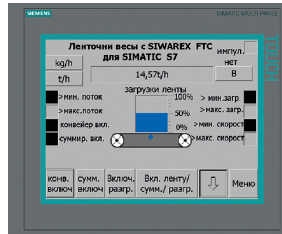
FTC conveyor scale
