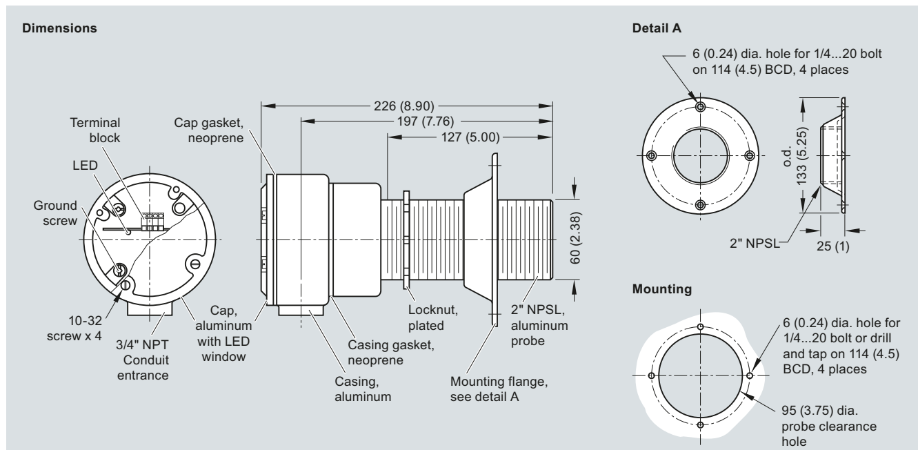
Millpulse 600 mounting, dimensions in mm (inch)
