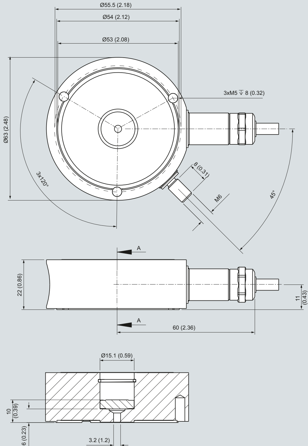
SIWAREX WL280 RN-S SA load cell (60 kg, 130 kg, 280 kg (132.28 lb, 286.60 lb, 617.29 lb)), dimensions in mm (inch)
