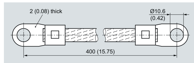
Grounding cable, dimensions in mm (inch)
