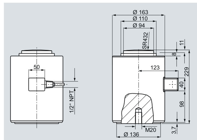
SIWAREX WL270 CP-S SC load cell, dimensions in mm (inch)
