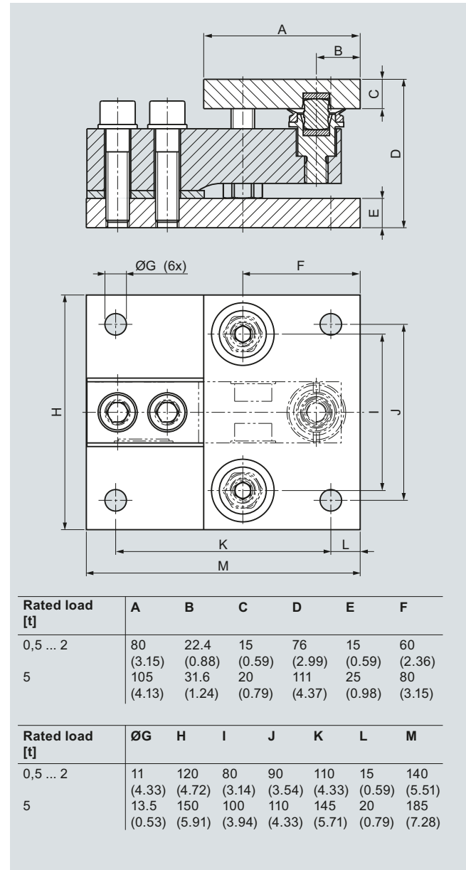
Compact mounting unit for SIWAREX WL230 SB-S SA load cells, dimensions in mm (inch)
