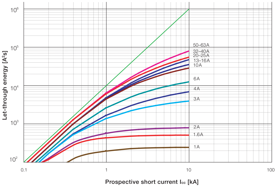
Miniature circuit breaker S400 B and D characteristics
