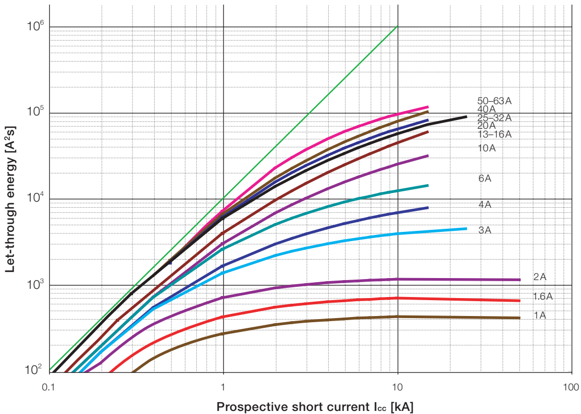
Miniature circuit breaker S400 C and K characteristics
